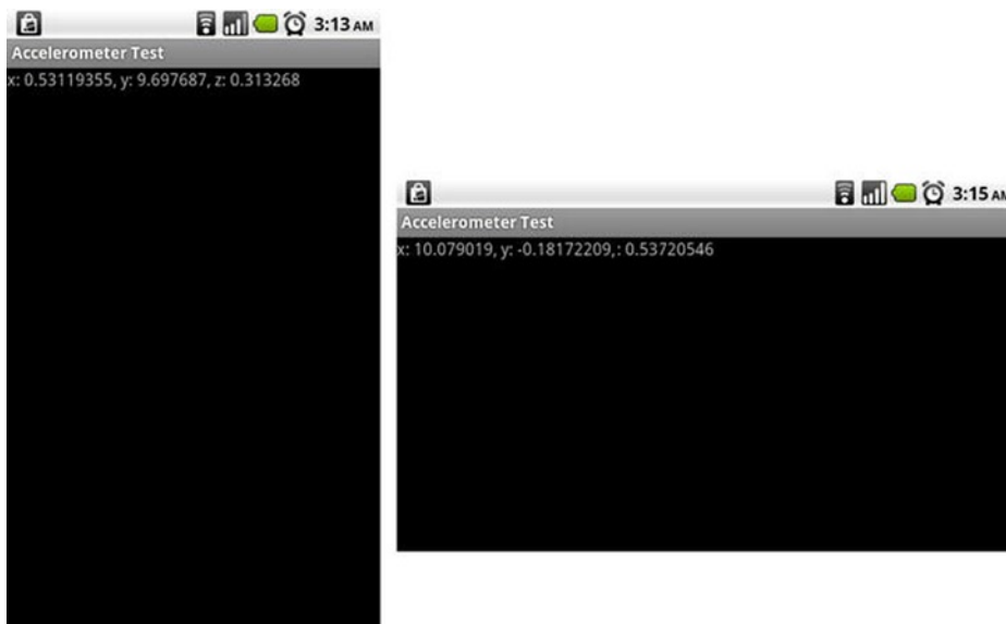
Figure 4-9. Accelerometer axes values in portrait mode (left) and landscape mode (right) when the device is held perpendicular to the ground
