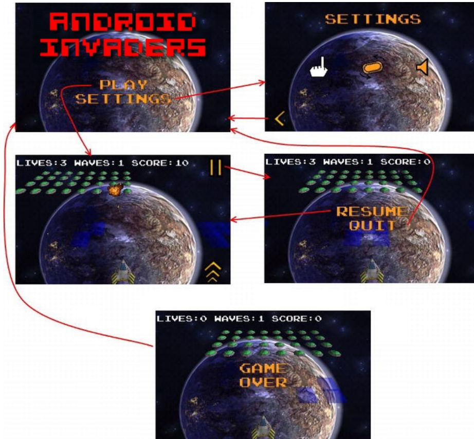
Figure 12-4. Screens and transitions of Android Invaders
