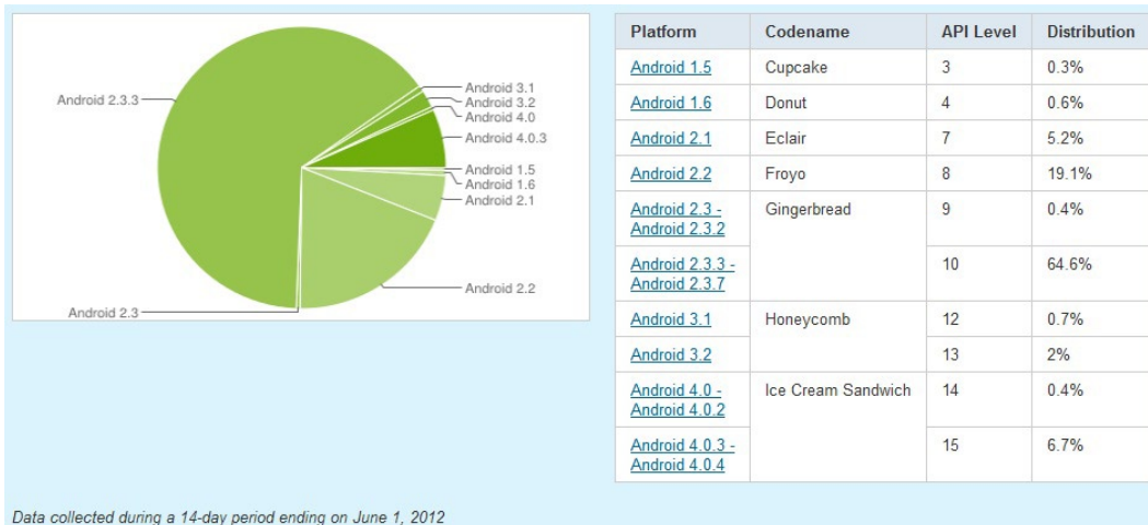
Figure 1-3. Android version distributions on August 1, 2012
