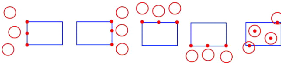
Figure 8-15. Overlap-testing a circle and a rectangle by finding the point on/in the rectangle that is closest to the circle
