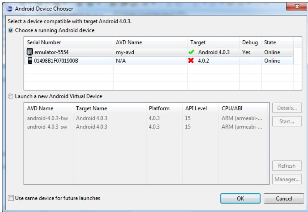
Figure 2-13. Choosing an emulator/device on which to run the application
