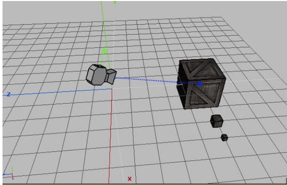
Figure 10-19. Our camera at position (3,3,0), looking at (0,0,-3)
