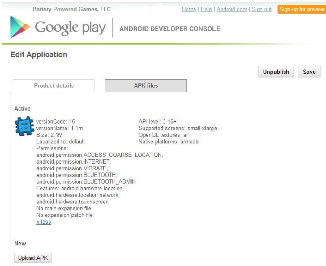
Figure 15-10. APK file management
