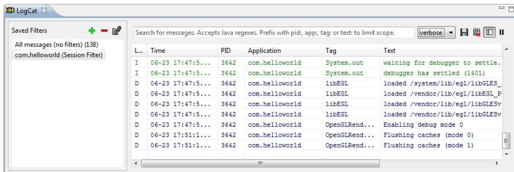
Figure 2-16. The LogCat view
