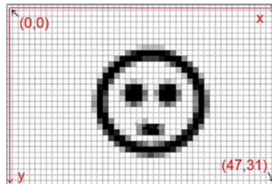
Figure 4-12. The coordinate system of a 48×32-pixel-wide screen
