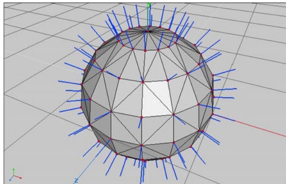
Figure 11-4. A sphere and its vertex normals
