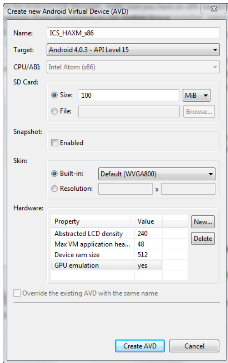
Figure 2-9. Creating the x86 AVD with GPU emulation enabled
